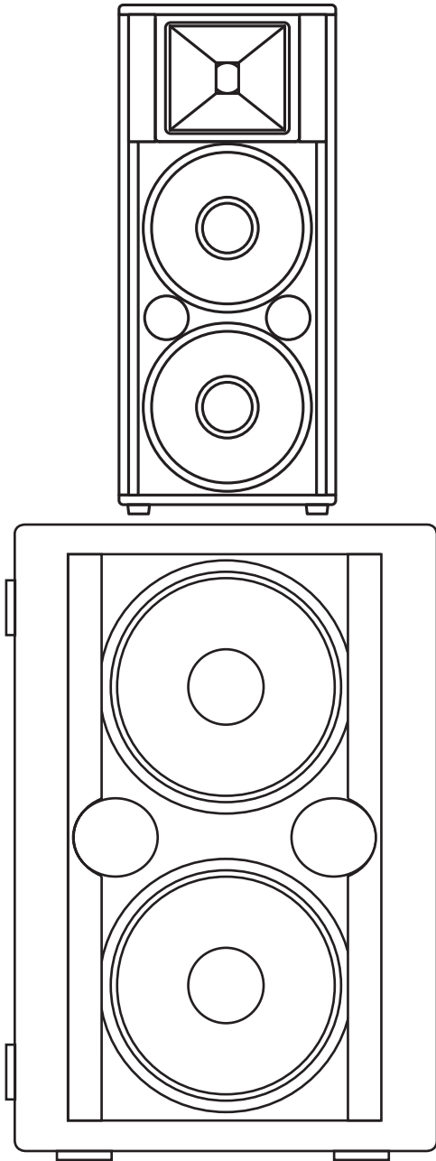
active sub (1500W) with built-in stereo electronic X-over (100Hz, 24dB/oct)
